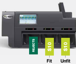
Fit Unfit
