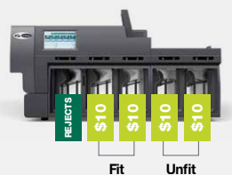
Fit Unfit
